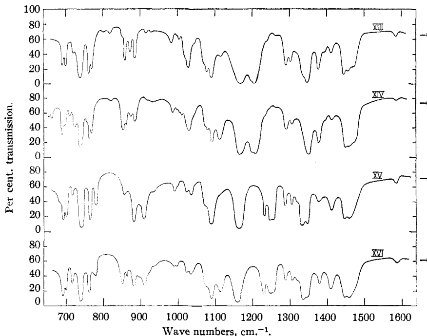
Fig. 3a, b.—Curve XIII, N,N' -dicarboethoxymethyl- N,N' -dibzenesulfonyldiaminomesitylene, m. p. 157–158°; Curve XIV, isomer of XIII, m. p. 116–119°; Curve XV, N,N' -dicarboxymethyl- N,N' -dibzenesulfonyldiaminomesitylene, m. p. 269–271°; Curve XVI, isomer of XV, m. p. 262.5–264.5°.
