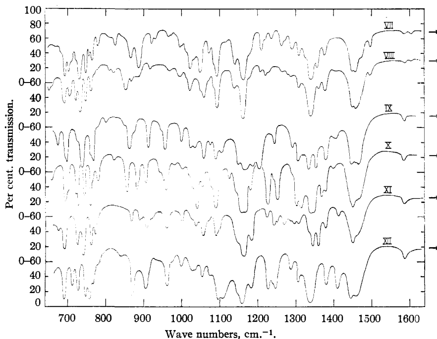
Fig. 2a, b.—Curve VII, N,N' -dibenzyl- N,N' -dibenzzenesulfonyldiaminomesitylene, m. p. 228–229°; Curve VIII, isomer of VII, m. p. 198–199°; Curve IX, N -ethyl- N' -carbethoxymethyl- N,N' -dibenzzenesulfonyldiaminomesitylene, m. p. 165–166°; Curve X, isomer of IX, m. p. 162.5–163.5°; Curve XI, N -ethyl- N' -carboxymethyl- N,N' -dibenzzenesulfonyldiaminomesitylene, m. p. 221–222°; Curve XII, isomer of XI, m. p. 203.5–204.5°.
