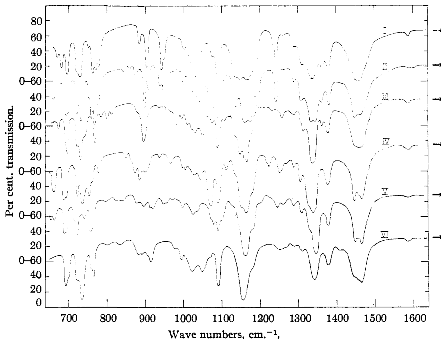
Fig. 1a, b.—Curve I, N,N' -diethyl- N,N' -dibenzzenesulfonyldiaminomesitylene, m. p. 212–212.5°; Curve II, isomer of I, m. p. 168–169°; Curve III, N,N' -dibutyl- N,N' -dibenzzenesulfonyldiaminomesitylene, m. p. 156.5–157.5°; Curve IV, isomer of III, m. p. 148–149°; Curve V, N,N' -didodecyl- N,N' -dibenzzenesulfonyldiaminomesitylene, m. p. 87–88°; Curve VI, isomer of V, m. p. 62.5–64.5°.
